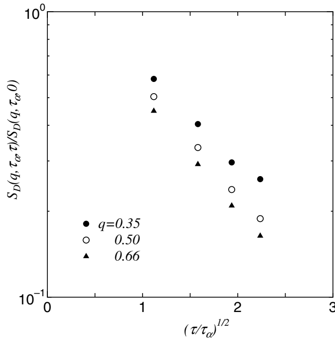
Figure 4. S_D(q, \tau_\alpha, \tau)/S_D(q, \tau_\alpha, 0) versus (\tau/\tau_\alpha)^{1/2} for q = 0.35, 0.5 , and 0.66 . This represents the decay of the heterogeneity structure.
