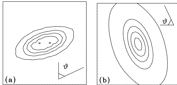
Figure 8. (a) Isointensity curves of g_s(\mathbf{r}) in equation (9) in the xy -plane ( -3.75 < x, y < 3.75 , z = 0 ). (b) Those of the incoherent structure factor S(\mathbf{q}) in equation (10) in the q_x q_y -plane ( -\pi < q_x, q_y < \pi , q_z = 0 ). The values for the isolines are 0.01 + 0.02n in (a) and 0.1 + 0.2n in (b) with n = 0, 1, \dots, 4 from outer to inner line. Here T = 0.2 , \dot{\gamma} = 10^{-4} , and the flow is in the horizontal ( x -) direction. \theta is the angle between the average chain shapes and the y -axis.
