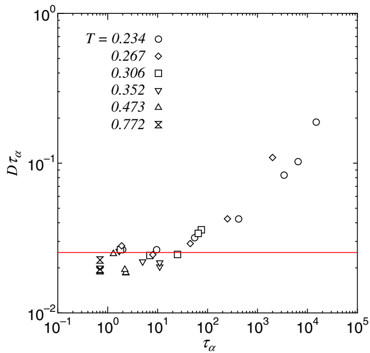
Figure 2. D\tau_\alpha versus \tau_\alpha . The solid line represents the Stokes–Einstein value D_{ES}\tau_\alpha = (2\pi)^{-2} .
