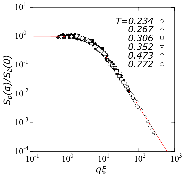
Figure 1. S_b(q)/S_b(0) on logarithmic scales for various T and \dot{\gamma} in 3D. Open and closed symbols represent results for \dot{\gamma} = 0 and \dot{\gamma} \neq 0 , respectively. The solid line is the OZ form 1/(1+x^2) with x = q\xi .
