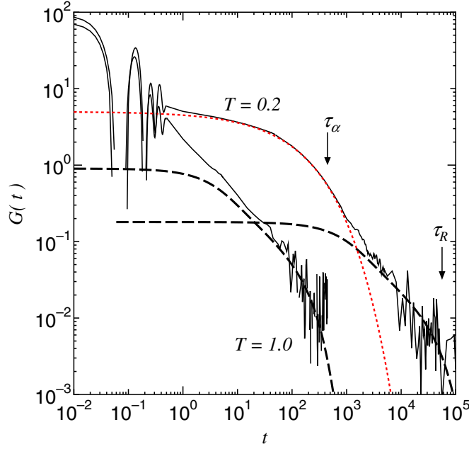
Figure 5. The stress relaxation function G(t) (thin solid lines) at T = 0.2 in a supercooled state and T = 1 in a normal-liquid state. It may be fitted to the stretched-exponential form (dotted line) at relatively short times and tends to the Rouse relaxation function G_R(t) (bold dashed lines) at long times.
