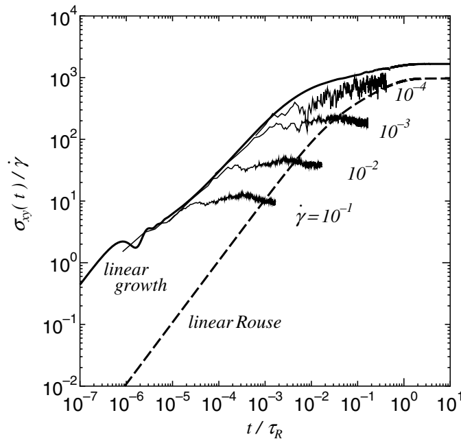
Figure 6. Shear stress divided by shear rate \dot{\gamma} = 10^{-1}, 10^{-2}, 10^{-3}, 10^{-4} (thin solid lines) versus t/\tau_R (where \tau_R = 6 \times 10^4 ) at T = 0.2 . The curves follow the linear growth function (bold solid line) for \dot{\gamma}t \lesssim 0.1 , but afterwards depart from it. The linear growth function in the Rouse model is also plotted (bold dashed line).
