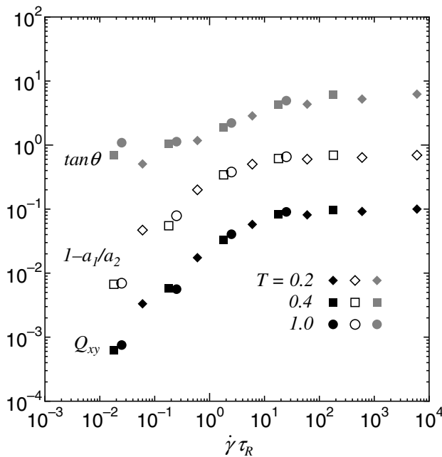
Figure 9. \tan \theta , 1 - a_1/a_2 , and Q_{xy} versus \dot{\gamma}\tau_R .
